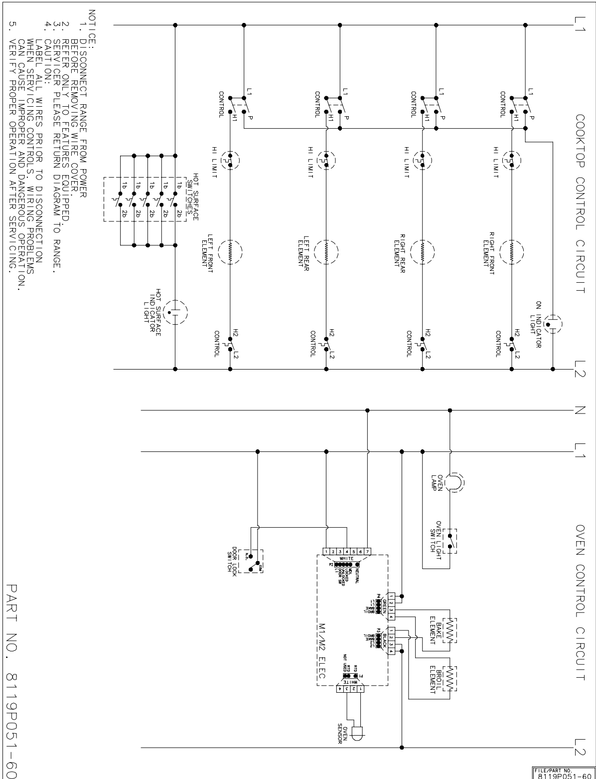
AER5712AA*, MER5751AA*, MER5752AA*, CER3725AA* Control Circuit
